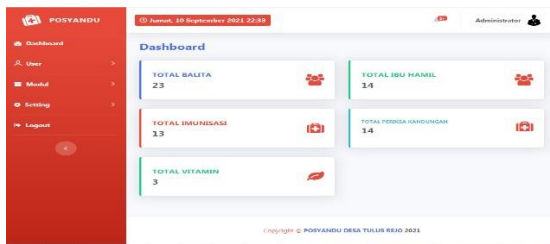
Gambar 4. Tampilan Dashboard
